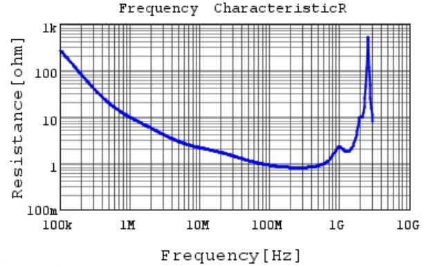
DE1B3KX471KA4BN01F R DCOV, 20degC
