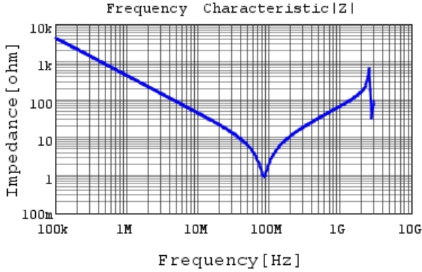
DE1B3KX471KA4BN01F |Z| DCOV, 20degC
