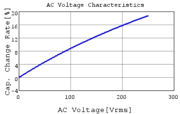
DE1B3KX471KA4BN01F C-AC Voltage capchange, I
