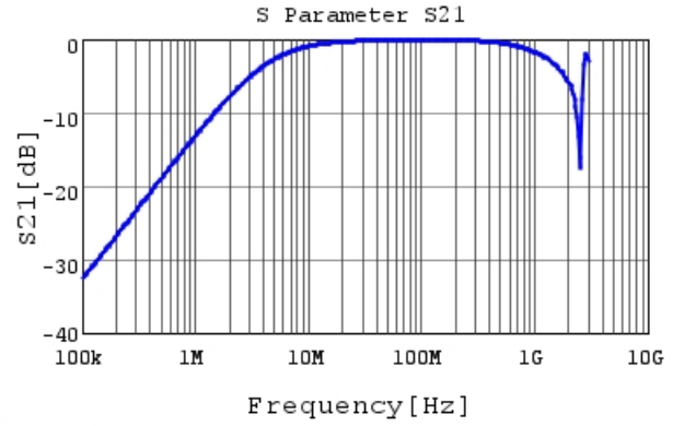
DE1B3KX471KA4BN01F S21 DCOV, 20degC
