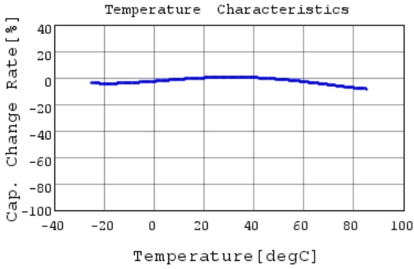
DE1B3KX471KA4BN01F C-Temp. capchange, DCOV,
