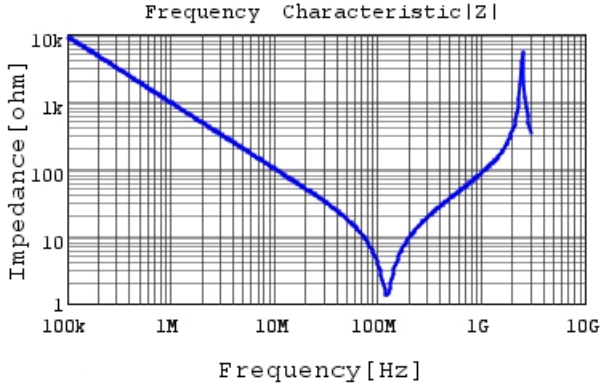
DE6B3KJ221KN3A |Z| DCOV, 20degC
