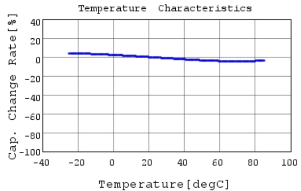
DE6B3KJ221KN3A C-Temp. capchange, DCOV, AC1V
