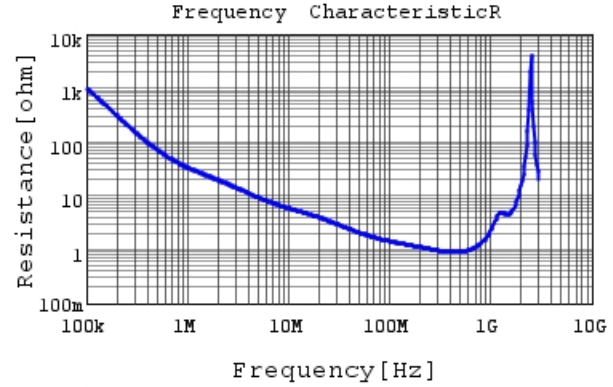
DE6B3KJ221KN3A R DCOV, 20degC
