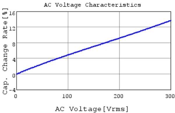
DE6B3KJ221KN3A C-AC Voltage capchange, DCOV,
