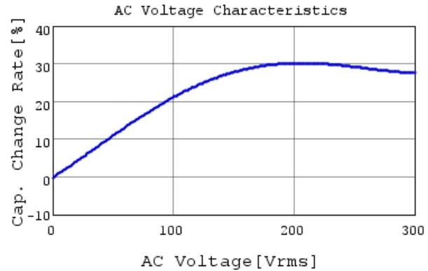
DE2E3SA222MN3AX02F C-AC Voltage capchange, I
