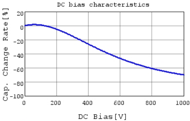
DE2E3SA222MN3AX02F C-DC bias capchange, 20.0
