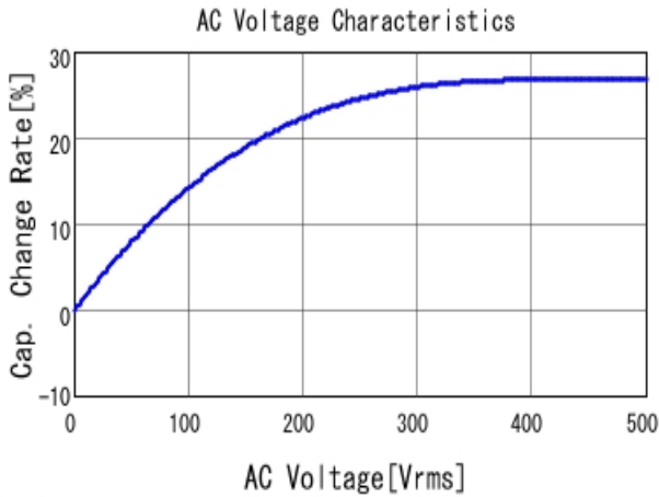
■ DE1E3RA102MA4BQ01F C-AC Voltage capchange, DCOV, 20.0
