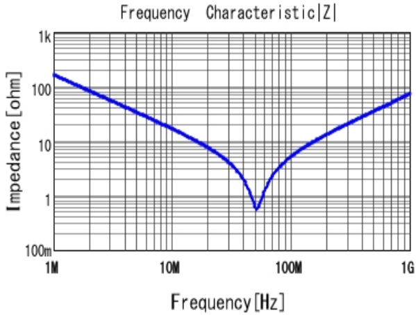
■ DE1E3RA102MA4BQ01F |Z| DCOV, 20degC
