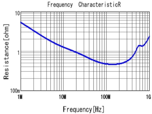
■ DE1E3RA102MA4BQ01F R DCOV, 20degC
