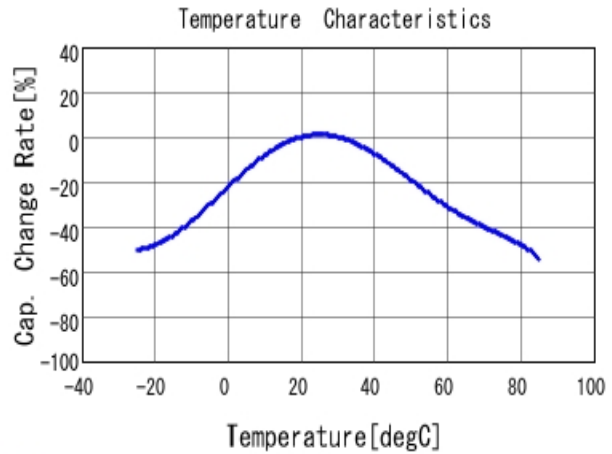
■ DE1E3RA102MA4BQ01F C-Temp. capchange, DCOV, AC1Vrms
