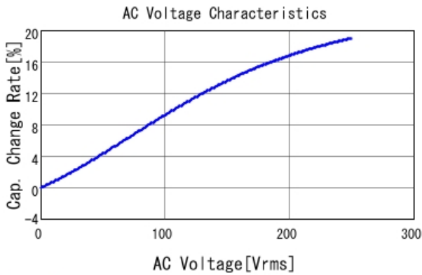
DE2B3SA151KN2AT01F C-AC Voltage capchange, DCOV, 2
