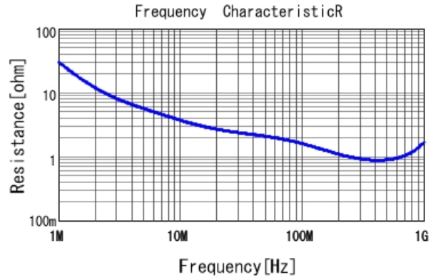
DE2B3SA151KN2AT01F R DCOV, 20degC
