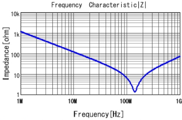
DE2B3SA151KN2AT01F |Z| DCOV, 20degC
