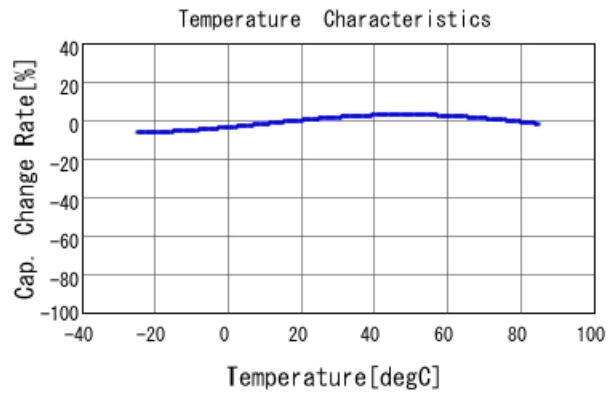
DE2B3SA151KN2AT01F C-Temp. capchange, DCOV, AC1Vrr
