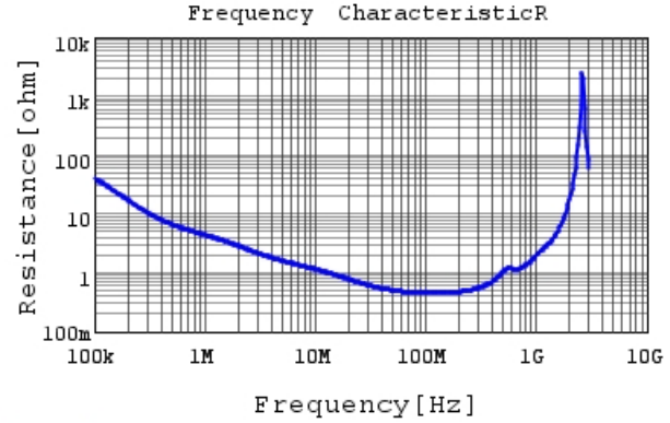
DE1E3KX152MJ4BP01F R DCOV, 20degC
