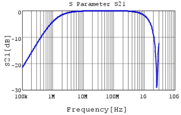
DE1E3KX152MJ4BP01F S21 DC0V, 20degC
