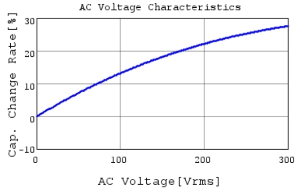
DE1E3KX152MJ4BP01F C-AC Voltage capchange, I
