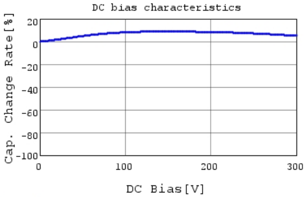
DE1E3KX152MJ4BP01F C-DC bias capchange, 20.0
