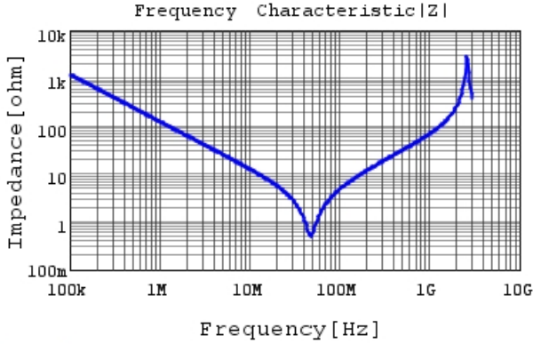
DE1E3KX152MJ4BP01F |Z| DCOV, 20degC
