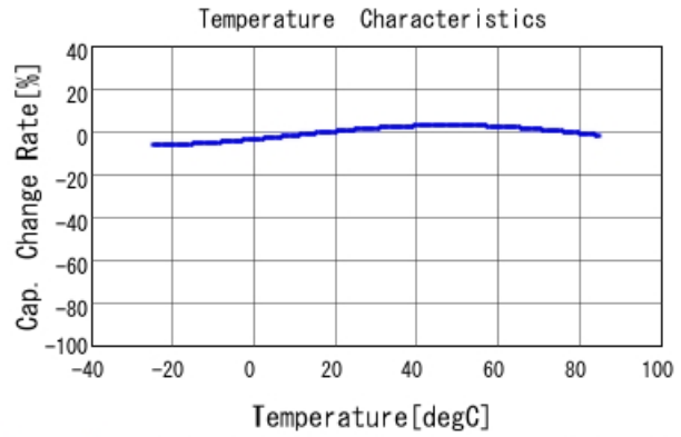
DE2B3SA101KN2AT01F C-Temp. capchange, DCOV, AC1Vrr
