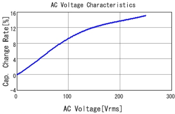
DE2B3SA101KN2AT01F C-AC Voltage capchange, DCOV, 2
