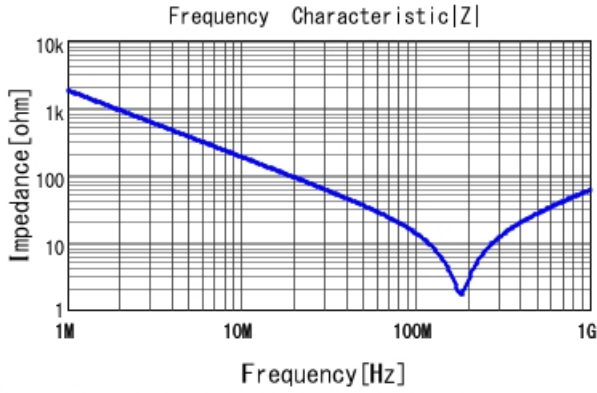
DE2B3SA101KN2AT01F |Z| DCOV, 20degC
