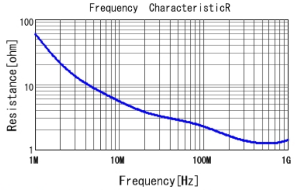
DE2B3SA101KN2AT01F R DCOV, 20degC
