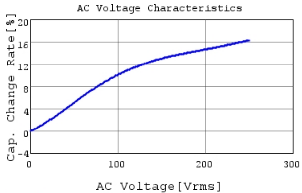
DE1B3RA151KJ4BN01F C-AC Voltage capchange, I
