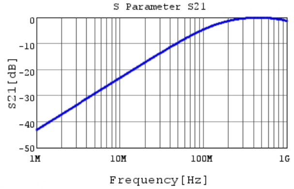
DE11XRA100KJ4BQ01F S21 DCOV, 20degC
