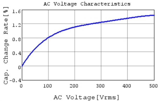
DE11XRA100KJ4BQ01F C-AC Voltage capchange, I
