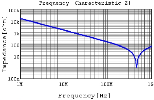
DE11XRA100KJ4BQ01F |Z| DC0V, 20degC
