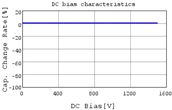
DE11XRA100KJ4BQ01F C-DC bias capchange, 20.0
