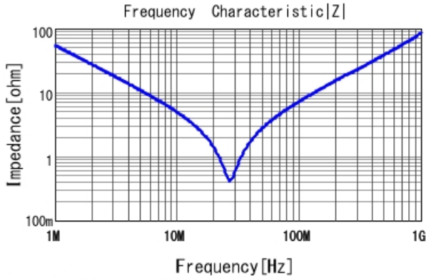
DE1E3RA332MA4BQ01F |Z| DCOV, 20degC
