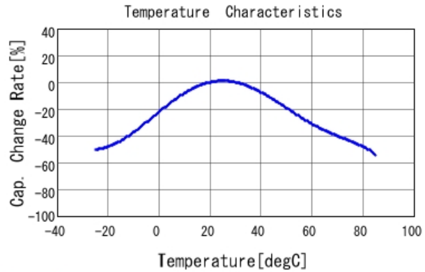
DE1E3RA332MA4BQ01F C-Temp. capchange, DCOV, AC1Vrr
