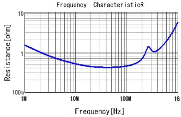
DE1E3RA332MA4BQ01F R DCOV, 20degC
