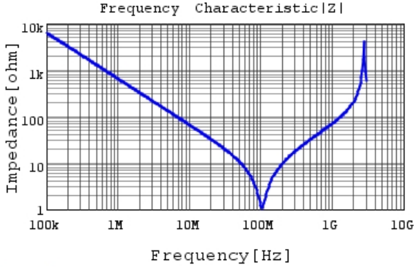
DE1B3KX331KB4BN01F |Z| DC0V, 20degC
