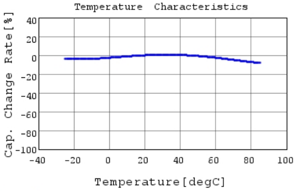
DE1B3KX331KB4BN01F C-Temp. capchange, DCOV,
