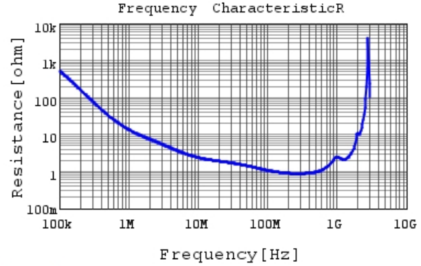
DE1B3KX331KB4BN01F R DC0V, 20degC
