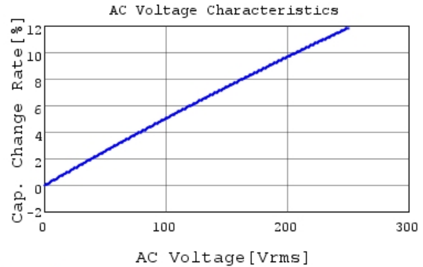
DE1B3KX331KB4BN01F C-AC Voltage capchange, I
