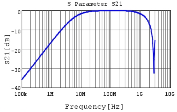
DE1B3KX331KB4BN01F S21 DCOV, 20degC
