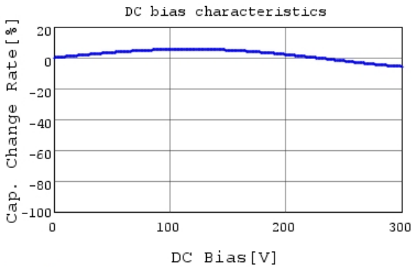
DE2E3KY222MB3BU02F C-DC bias capchange, 20.0
