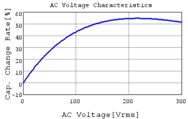
DE2E3KY222MB3BU02F C-AC Voltage capchange, I
