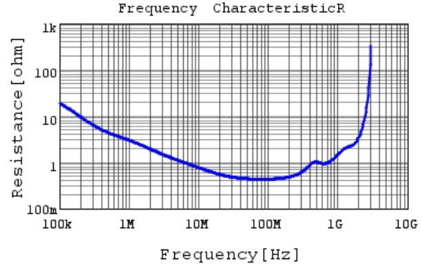
DE2E3KY222MB3BU02F R DC0V, 20degC
