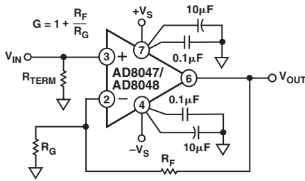
Figure 3. Noninverting Operation
