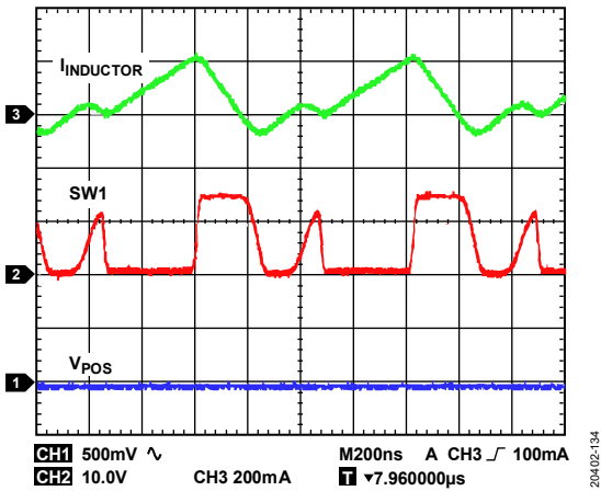
Figure 34. Boost Regulator Discontinuous Conduction Mode Operation Showing I_{INDUCTOR} , Switch Node Voltage, and Output Ripple, V_{IN} = 5V , V_{POS} = 15V , I_{LOAD1} = 6mA , f_{SW} = 2.4MHz , T_A = 25^\circ C
