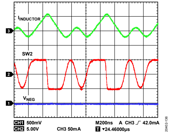
Figure 37. Inverting Regulator Discontinuous Conduction Mode Operation Showing I_{INDUCTOR} , Switch Node Voltage, and Output Ripple, V_{IN} = +5V , V_{NEG} = -5V , I_{LOAD2} = 6mA , f_{SW} = 2.4MHz , T_A = 25^\circ C
