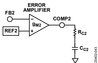
Figure 45. Compensation Component
