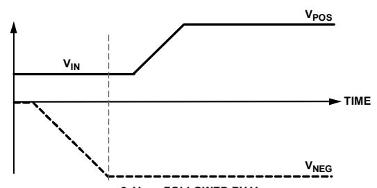
Figure 42. Sequential Enable Mode
