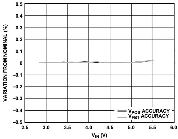
Figure 16. Boost Regulator Line Regulation, V_{POS} = 15\text{ V} , f_{SW} = 1.2\text{ MHz} , 15\text{ mA Load} , T_A = 25^\circ\text{C}
