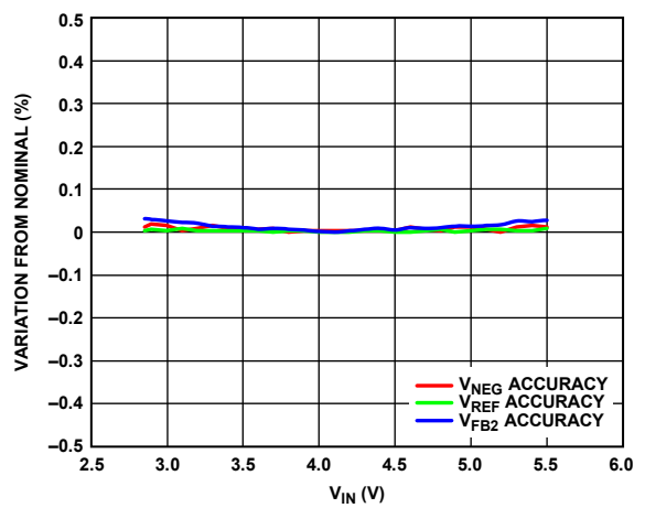
Figure 19. Inverting Regulator Line Regulation, V_{NEG} = -15\text{ V} , f_{SW} = 1.2\text{ MHz} , 15\text{ mA Load} , T_A = 25^\circ\text{C}
