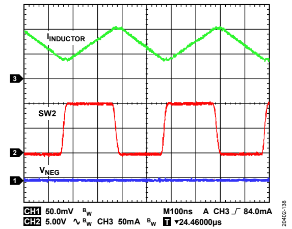
Figure 38. Inverting Regulator Continuous Conduction Mode Operation Showing I_{INDUCTOR} , Switch Node Voltage, and Output Ripple, V_{IN} = +5V , V_{NEG} = -5V , I_{LOAD2} = 35mA , f_{SW} = 2.4MHz , T_A = 25^\circ C
