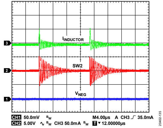
Figure 36. Inverting Regulator Skip Mode Operation Showing I_{INDUCTOR} , Switch Node Voltage, and Output Ripple, V_{IN} = +5V , V_{NEG} = -5V , I_{LOAD2} = 0mA , f_{SW} = 2.4MHz , T_A = 25^\circ C
