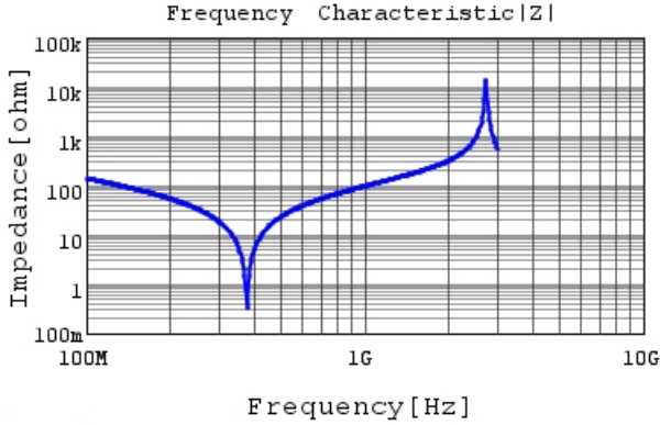
DE21XKY220JA2BM01F |Z| DCOV, 20degC
