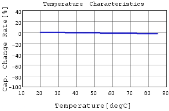
DE21XKY220JA2BM01F C-Temp. capchange, DCOV,
