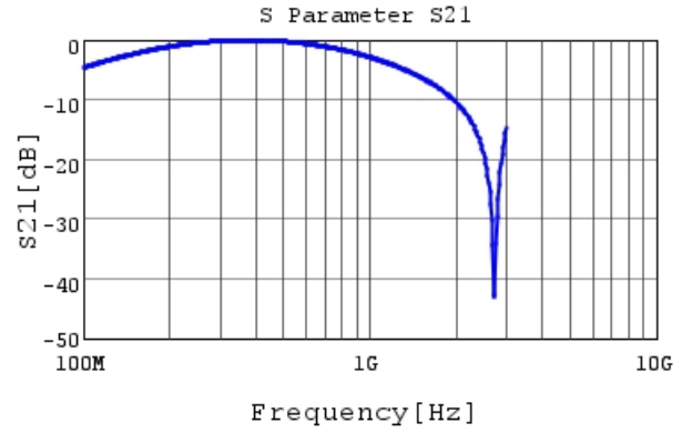
DE21XKY220JA2BM01F S21 DCOV, 20degC
