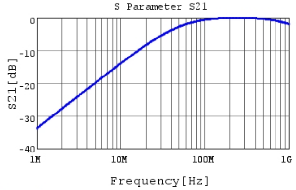
DE11XRA330KN4AQ01F S21 DCOV, 20degC
