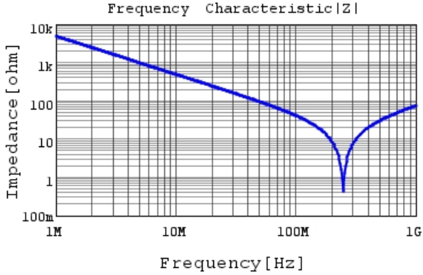
DE11XRA330KN4AQ01F |Z| DC0V, 20degC
