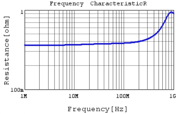
DE11XRA330KN4AQ01F R DC0V, 20degC
