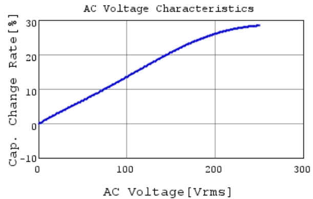
DE1E3RA472MA4BN01F C-AC Voltage capchange, I
