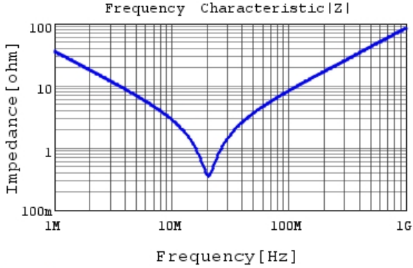
DE1E3RA472MA4BN01F |Z| DC0V, 20degC
