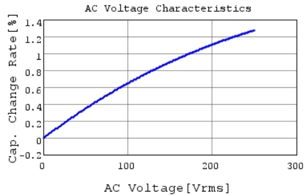
DE11XKX470JA4BC05F C-AC Voltage capchange, I
