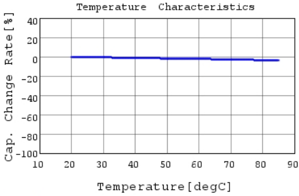
DE11XKX470JA4BC05F C-Temp. capchange, DCOV,
