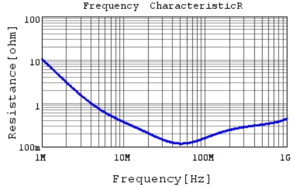
DE11XKX470JA4BC05F R DC0V, 20degC
