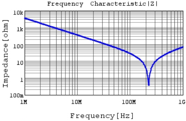
DE11XKX470JA4BC05F |Z| DC0V, 20degC
