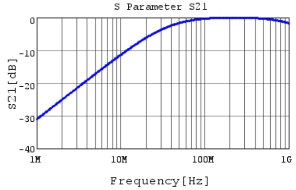
DE11XKX470JA4BC05F S21 DCOV, 20degC
