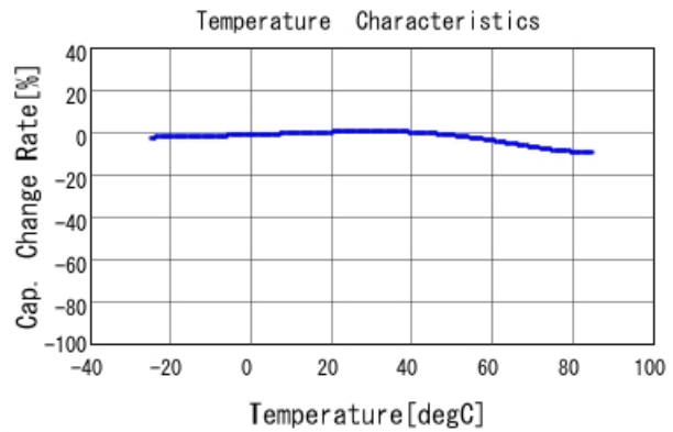
DE2B3SA221KN3AX02F C-Temp. capchange, DCOV, AC1Vrr
