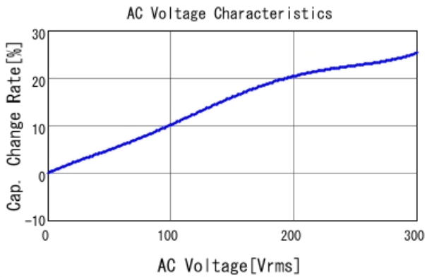
DE2B3SA221KN3AX02F C-AC Voltage capchange, DCOV, 2
