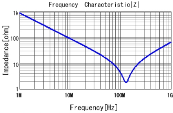
DE2B3SA221KN3AX02F |Z| DCOV, 20degC
