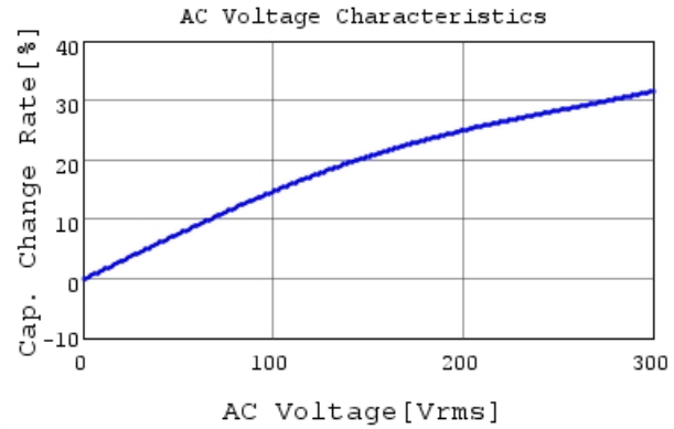
DE2B3SA681KA3BX02F C-AC Voltage capchange, I
