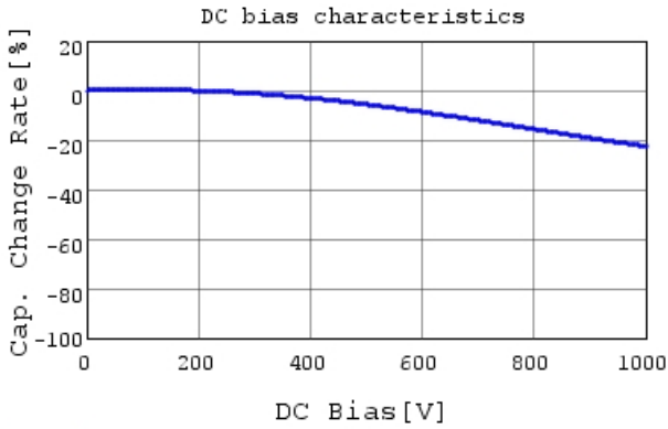
DE2B3SA681KA3BX02F C-DC bias capchange, 20.0
