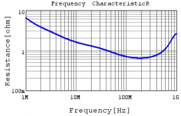
DE2B3SA681KA3BX02F R DC0V, 20degC
