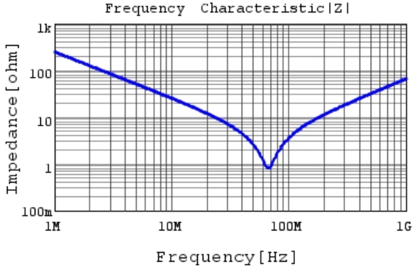
DE2B3SA681KA3BX02F |Z| DC0V, 20degC
