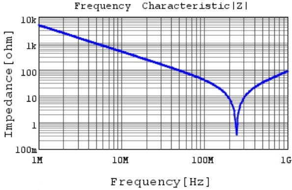
DE11XRA330KJ4BN01F |Z| DCOV, 20degC
