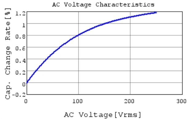
DE11XRA330KJ4BN01F C-AC Voltage capchange, I
