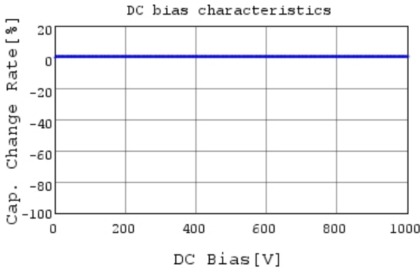
DE11XRA330KJ4BN01F C-DC bias capchange, 20.0
