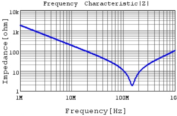
DE1B3RA101KN4AN01F |Z| DCOV, 20degC
