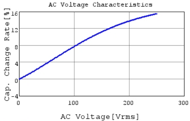
DE1B3RA101KN4AN01F C-AC Voltage capchange, I
