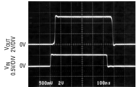
Output-Overload Recovery
