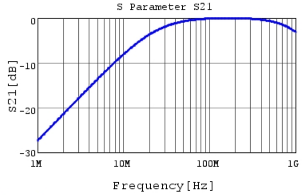
DE11XRA680KJ4BP01F S21 DCOV, 20degC
