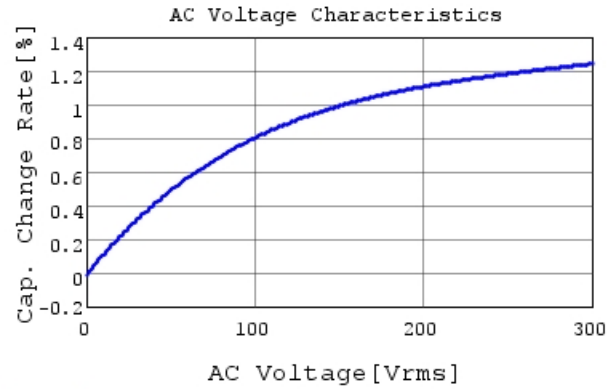
DE11XRA680KJ4BP01F C-AC Voltage capchange, I
