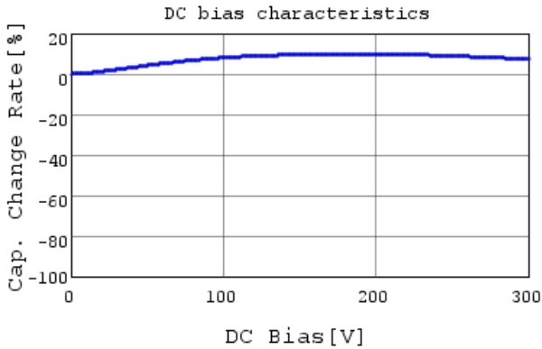
DE1E3KX472MA4BP01F C-DC bias capchange, 20.0
