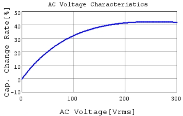
DE1E3KX472MA4BP01F C-AC Voltage capchange, I
