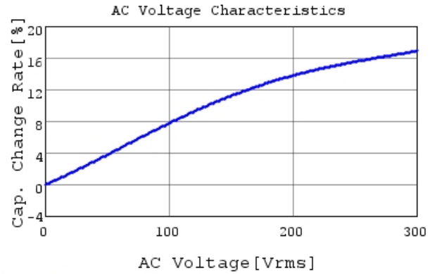
DE1B3RA101KN4AP01F C-AC Voltage capchange, I
