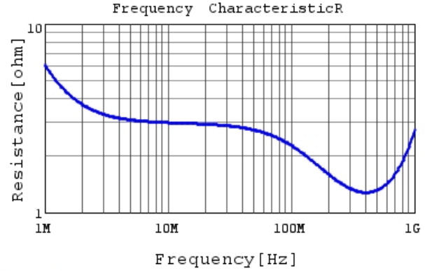
DE1B3RA101KN4AP01F R DCOV, 20degC
