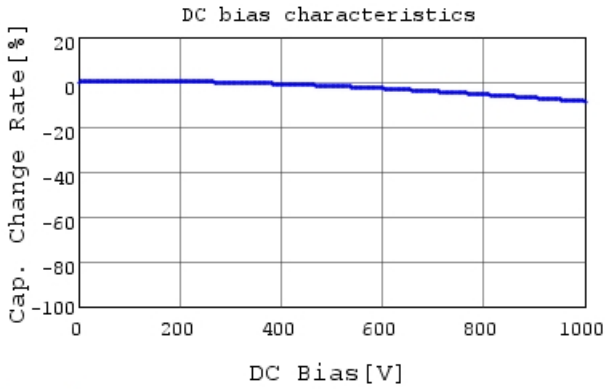
DE1B3RA101KN4AP01F C-DC bias capchange, 20.0
