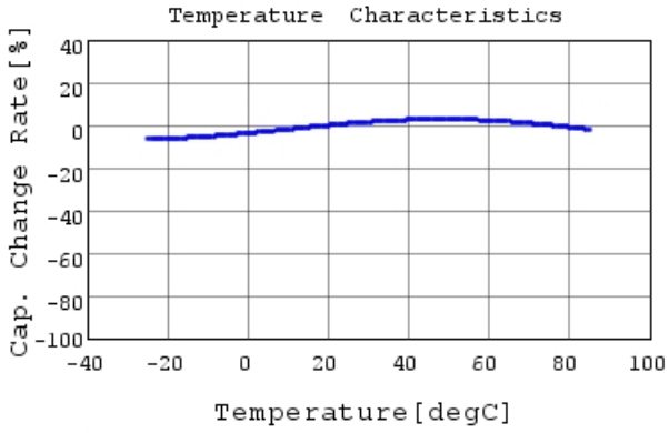
DE1B3RA101KN4AP01F C-Temp. capchange, DCOV,
