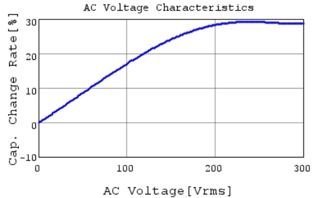
DE2E3SA472MA3BX02F C-AC Voltage capchange, I
