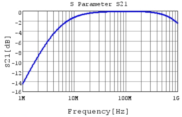
DE1B3RB331KA4BR01F S21 DCOV, 20degC
