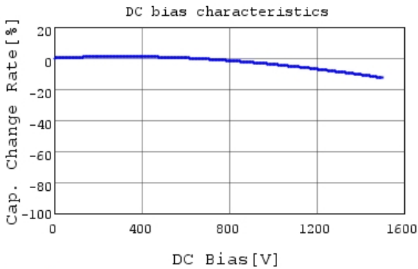
DE1B3RB331KA4BR01F C-DC bias capchange, 20.0
