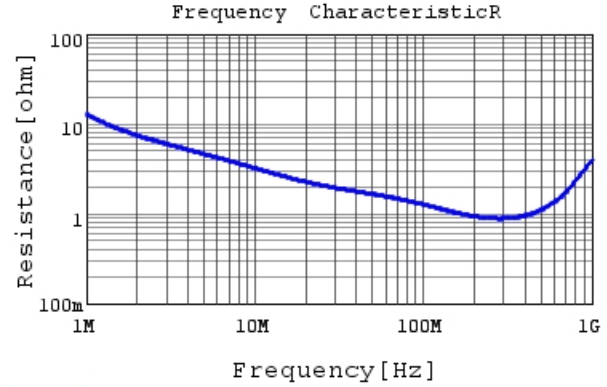
DE1B3RB331KA4BR01F R DC0V, 20degC
