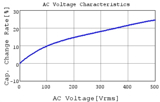
DE1B3RB331KA4BR01F C-AC Voltage capchange, I
