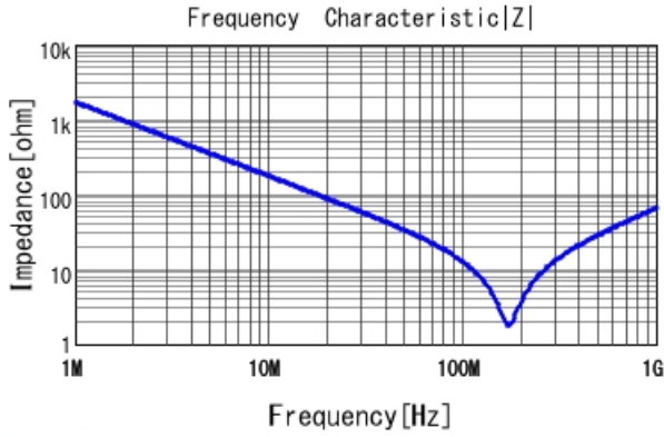
DE2B3SA101KN3AY02F |Z| DCOV, 20degC
