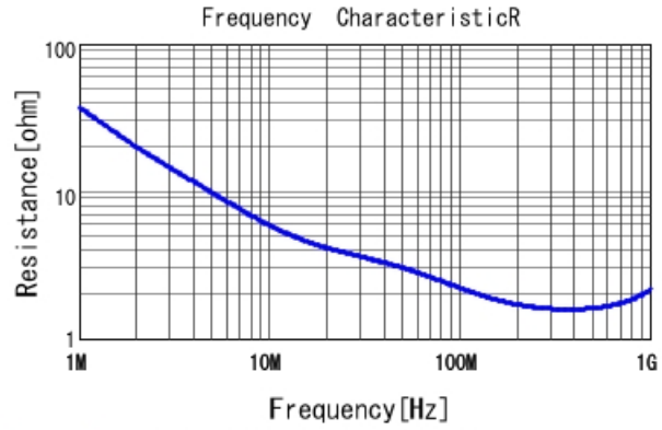
DE2B3SA101KN3AY02F R DCOV, 20degC
