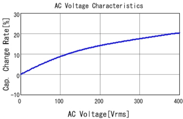
DE2B3SA101KN3AY02F C-AC Voltage capchange, DCOV, 2
