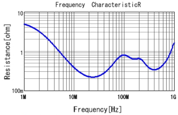
DE11XRA150KJ4BN01F R DCOV, 20degC
