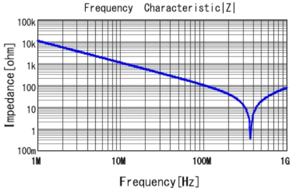
DE11XRA150KJ4BN01F |Z| DCOV, 20degC
