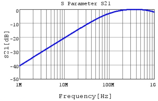
DE11XRA150KJ4BP01F S21 DCOV, 20degC
