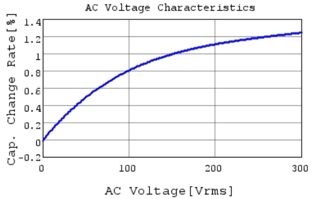
DE11XRA150KJ4BP01F C-AC Voltage capchange, I
