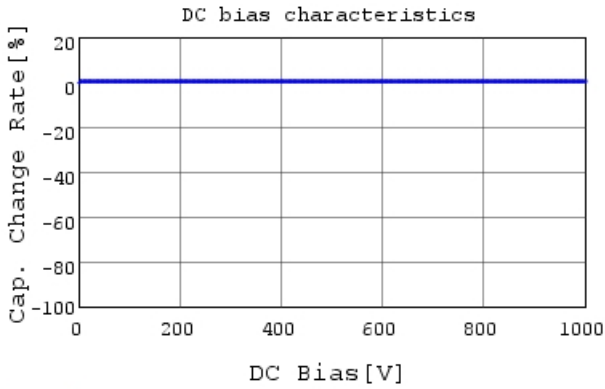
DE11XRA150KJ4BP01F C-DC bias capchange, 20.0
