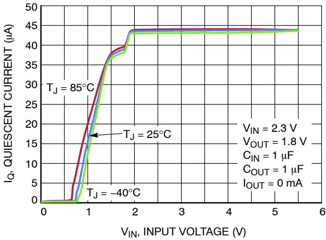
Figure 11. Quiescent Current vs. Input Voltage - V_{OUT} = 1.8 V
