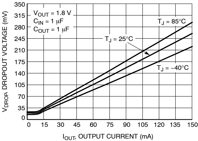
Figure 13. Dropout Voltage vs. Load Current - V_{OUT} = 1.8 V
