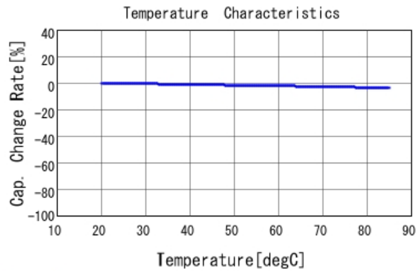
DE11XRA680KN4AN01F C-Temp. capchange, DCOV, AC1Vrr
