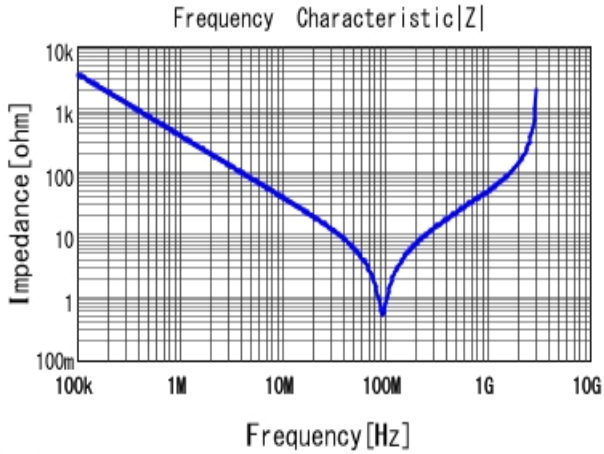
■ DE2B3KY471KN2AM01F |Z| DCOV, 20degC
