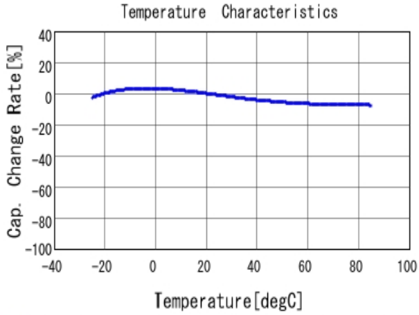
■ DE2B3KY471KN2AM01F C-Temp. capchange, DCOV, AC1Vrms
