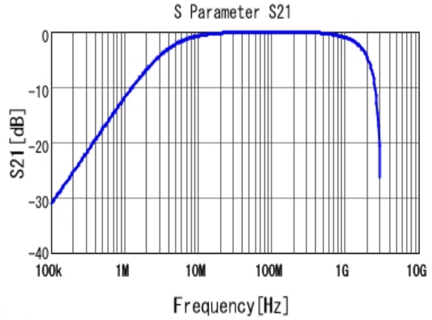
■ DE2B3KY471KN2AM01F S21 DCOV, 20degC
