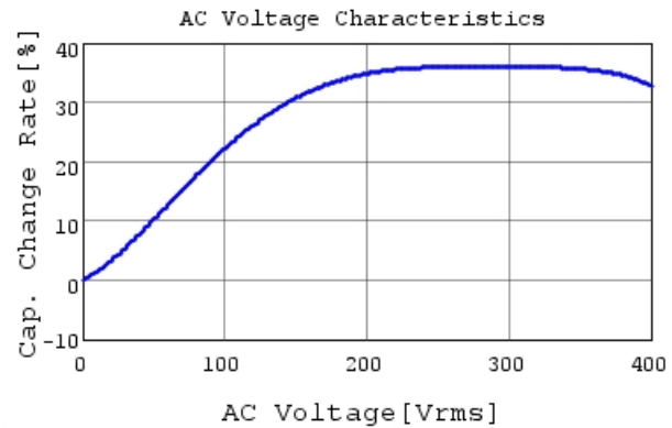
DE2E3SA102MA3BY02F C-AC Voltage capchange, I
