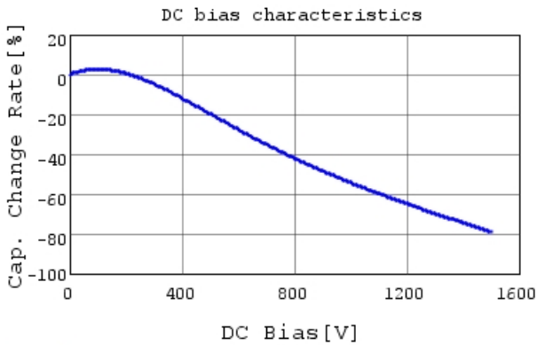
DE2E3SA102MA3BY02F C-DC bias capchange, 20.0
