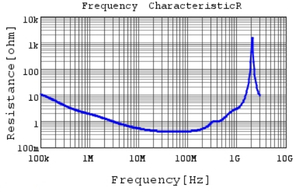
DE6E3KJ332MB3B R DCOV, 20degC
