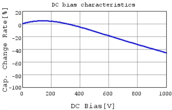
DE6E3KJ332MB3B C-DC bias capchange, 20.0degC
