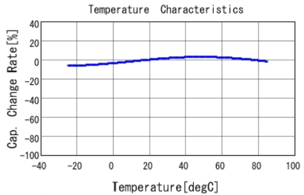
DE2B3SA101KJ3BT02F C-Temp. capchange, DCOV, AC1Vrr
