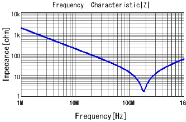
DE2B3SA101KJ3BT02F |Z| DCOV, 20degC
