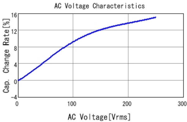
DE2B3SA101KJ3BT02F C-AC Voltage capchange, DCOV, 2
