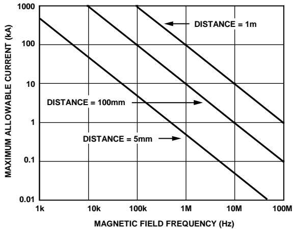
Figure 17. Maximum Allowable Current for Various Current-to-ADuM1300/ADuM1301 Spacings
