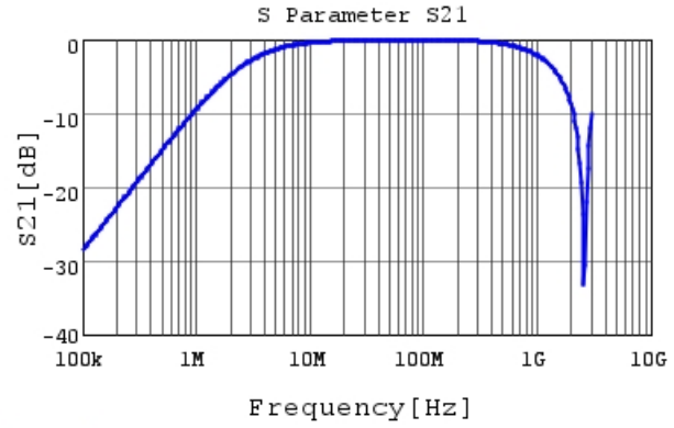
DE1B3KX681KB4BP01F S21 DCOV, 20degC
