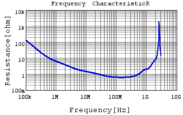
DE1B3KX681KB4BP01F R DCOV, 20degC
