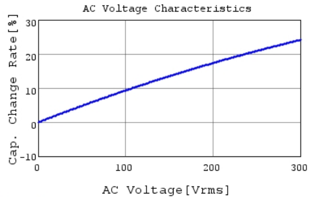
DE1B3KX681KB4BP01F C-AC Voltage capchange, I
