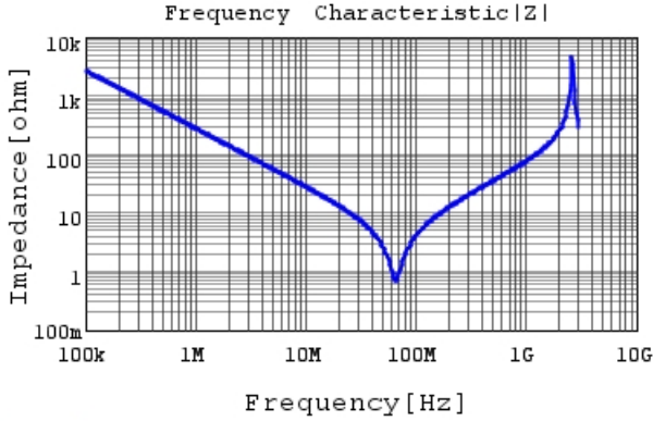
DE1B3KX681KB4BP01F |Z| DCOV, 20degC
