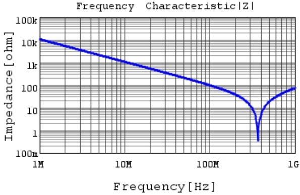
DE11XRA150KA4BN01F |Z| DCOV, 20degC
