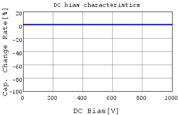
DE11XRA150KA4BN01F C-DC bias capchange, 20.0
