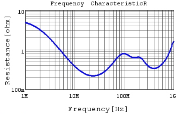
DE11XRA150KA4BN01F R DCOV, 20degC
