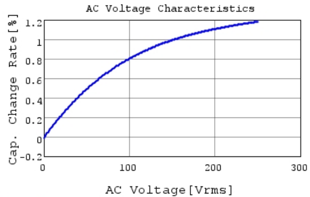
DE11XRA150KA4BN01F C-AC Voltage capchange, I
