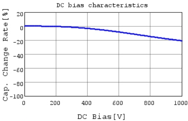
DE2B3SA471KJ2BT01F C-DC bias capchange, 20.0
