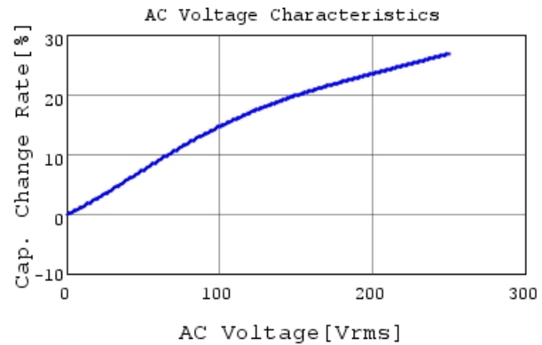
DE2B3SA471KJ2BT01F C-AC Voltage capchange, I
