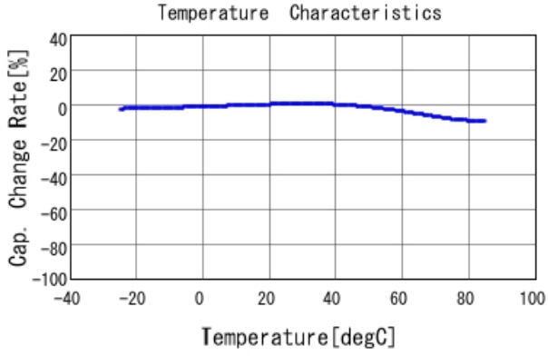
DE1B3RA471KJ4BN01F C-Temp. capchange, DCOV, AC1Vrrr
