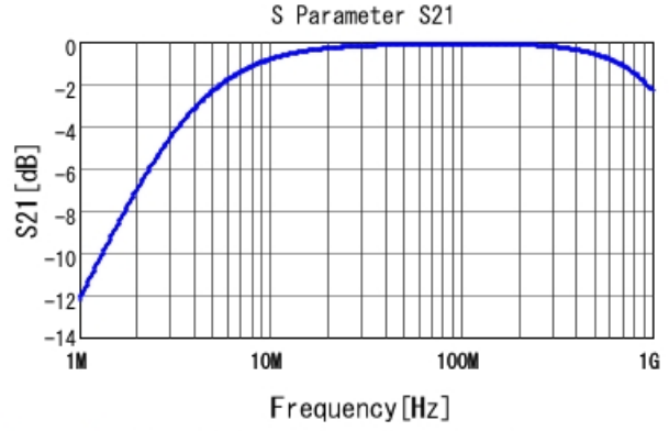
DE1B3RA471KJ4BN01F S21 DCOV, 20degC
