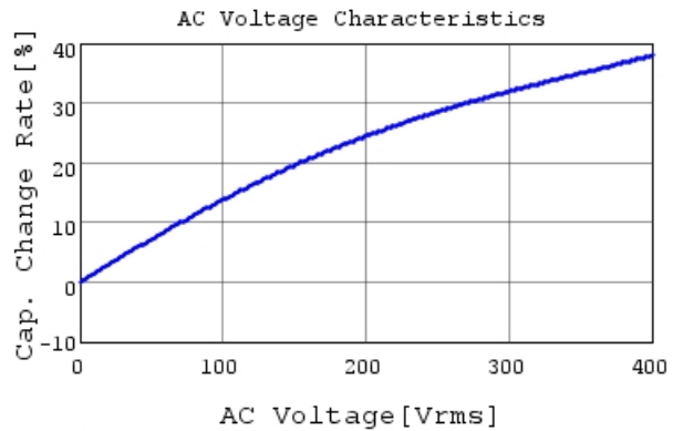
DE2B3SA471KA3BY02F C-AC Voltage capchange, I
