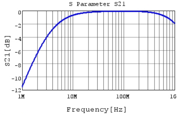
DE2B3SA471KA3BY02F S21 DCOV, 20degC
