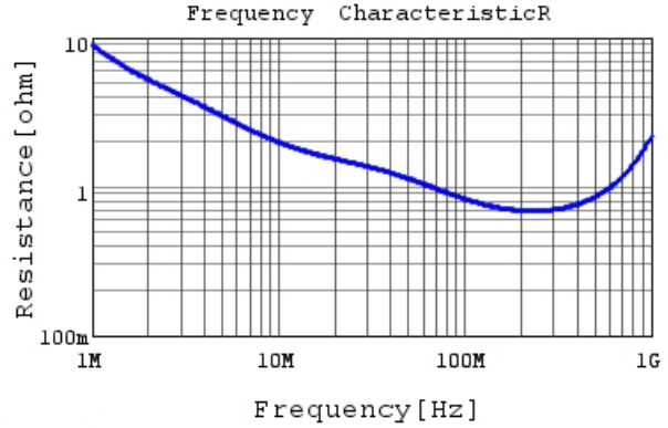
DE2B3SA471KA3BY02F R DC0V, 20degC
