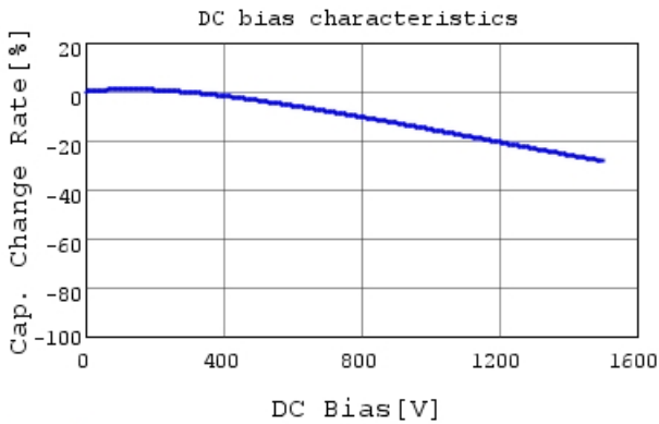
DE2B3SA471KA3BY02F C-DC bias capchange, 20.0
