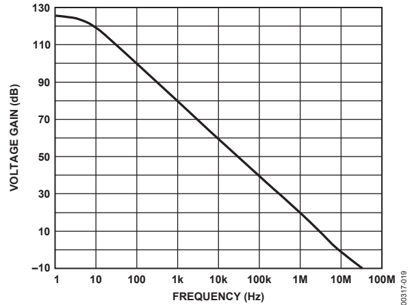
Figure 19. Open-Loop Gain vs. Frequency
