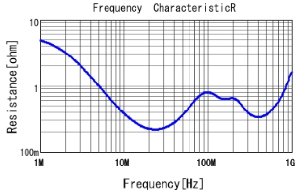
DE11XRA150KA4BP01F R DCOV, 20degC
