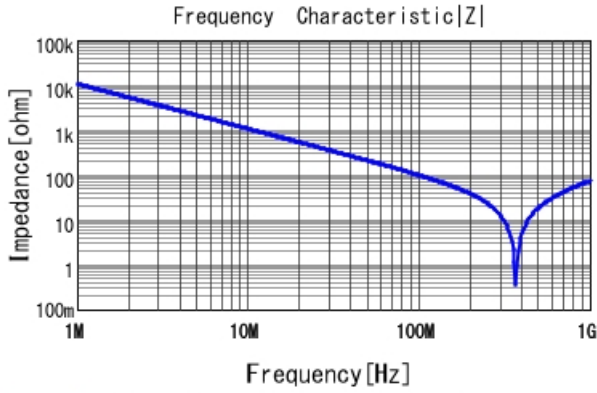
DE11XRA150KA4BP01F |Z| DCOV, 20degC
