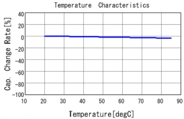
DE11XRA150KA4BP01F C-Temp. capchange, DCOV, AC1Vrr
