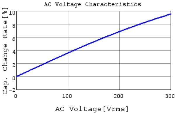
DE6B3KJ101KA3B C-AC Voltage capchange, DCOV,
