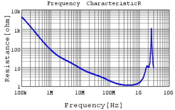
DE6B3KJ101KA3B R DCOV, 20degC
