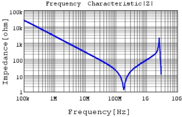
DE6B3KJ101KA3B |Z| DCOV, 20degC
