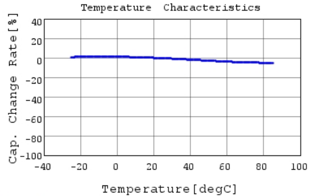
DE6B3KJ101KA3B C-Temp. capchange, DCOV, AC1V
