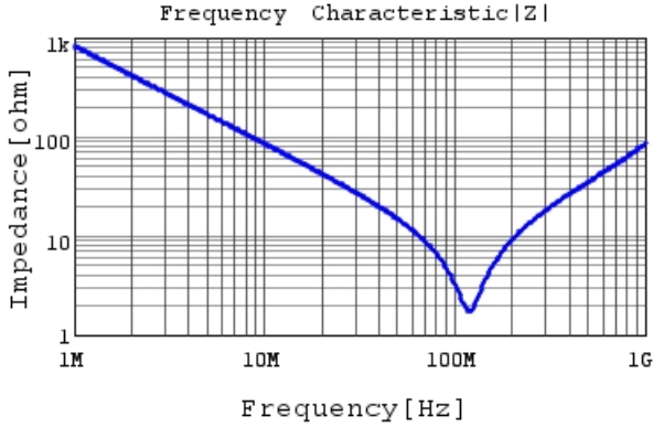
DE1B3RA221KJ4BN01F |Z| DC0V, 20degC
