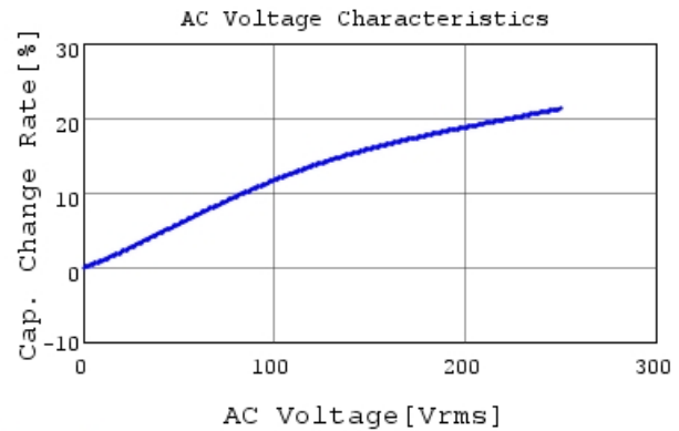
DE1B3RA221KJ4BN01F C-AC Voltage capchange, I
