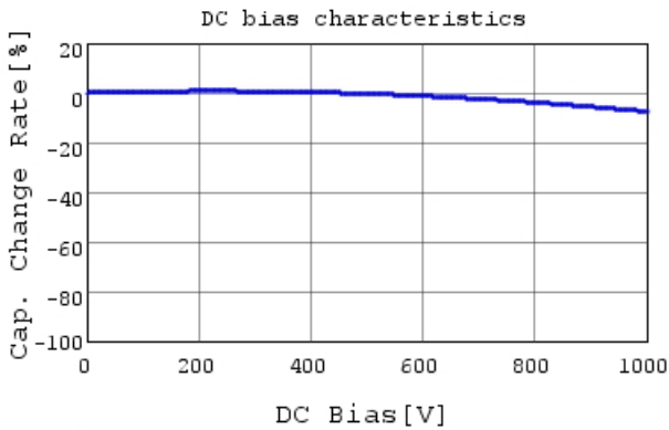
DE1B3RA221KJ4BN01F C-DC bias capchange, 20.0
