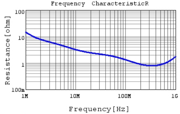
DE1B3RA331KA4BP01F R DC0V, 20degC
