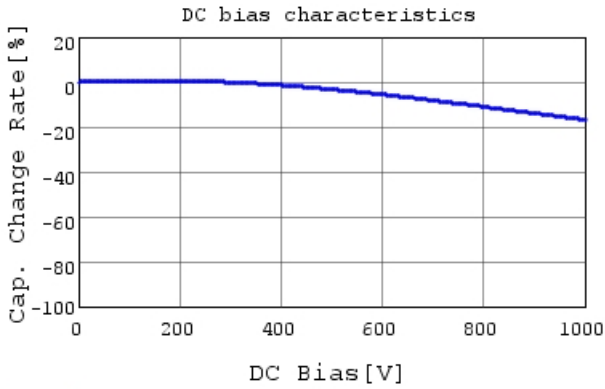
DE1B3RA331KA4BP01F C-DC bias capchange, 20.0
