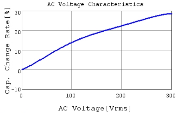
DE1B3RA331KA4BP01F C-AC Voltage capchange, I
