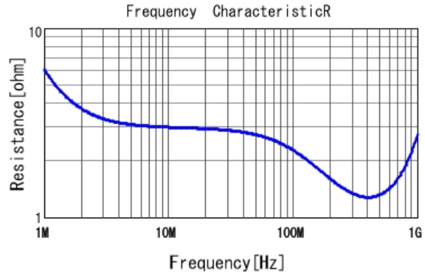
DE1B3RA101KJ4BP01F R DCOV, 20degC
