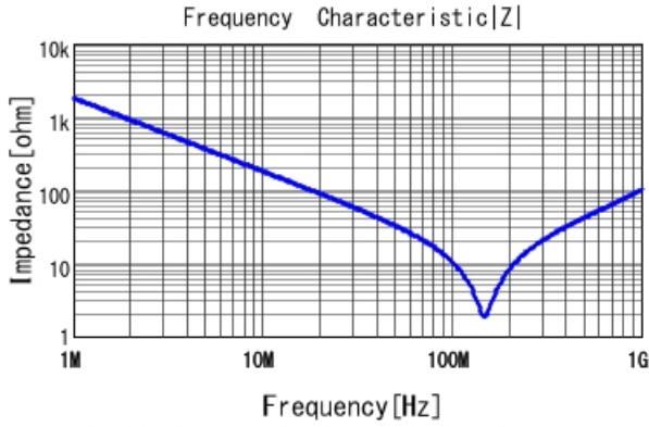
DE1B3RA101KJ4BP01F |Z| DCOV, 20degC
