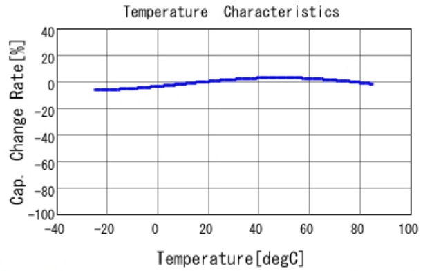
DE1B3RA101KJ4BP01F C-Temp. capchange, DCOV, AC1Vrrr
