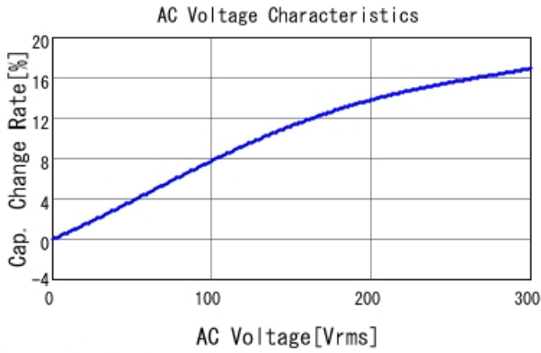
DE1B3RA101KJ4BP01F C-AC Voltage capchange, DCOV, 2
