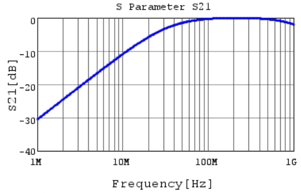
DE11XRA470KJ4BQ01F S21 DCOV, 20degC
