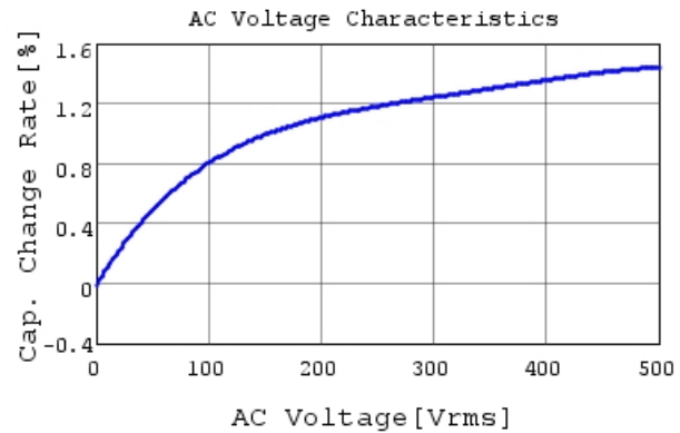
DE11XRA470KJ4BQ01F C-AC Voltage capchange, I
