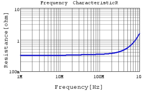
DE11XRA470KJ4BQ01F R DC0V, 20degC
