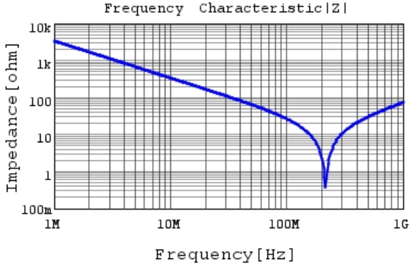
DE11XRA470KJ4BQ01F |Z| DC0V, 20degC
