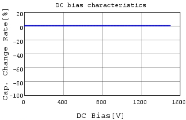
DE11XRA470KJ4BQ01F C-DC bias capchange, 20.0
